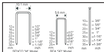
Nail specification
